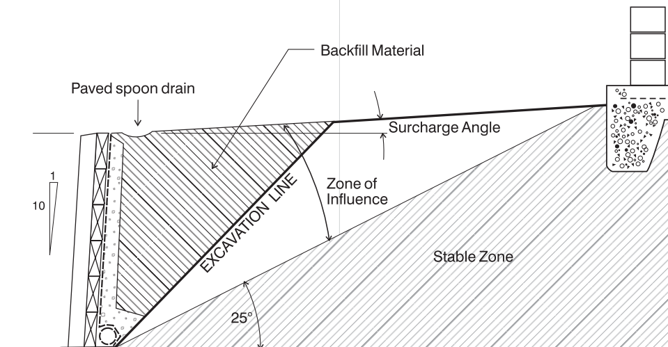
Figure 3 - Stable zone
